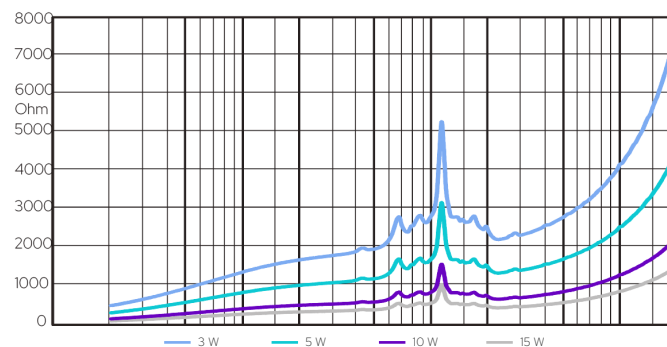
Impedance
