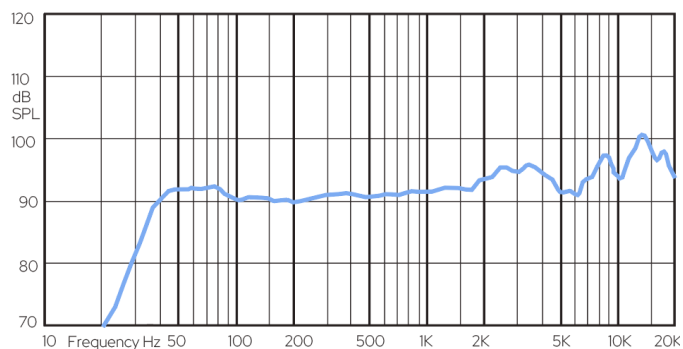
Frequency response
