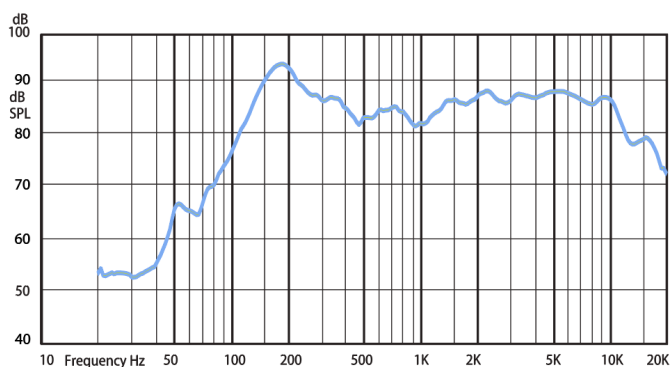
Frequency response
