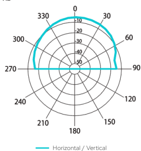
Horizontal/vertical polar diagrams
