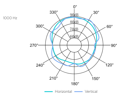
Horizontal/vertical polar diagrams
