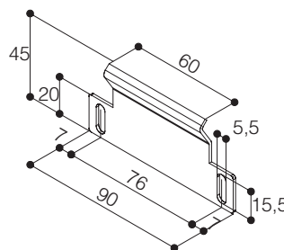
WALL BRACKET
