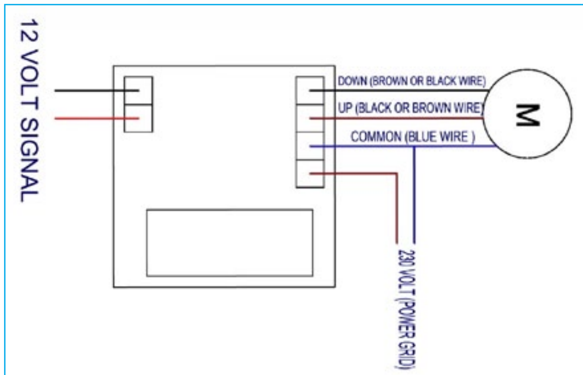
WIRING DIAGRAM
